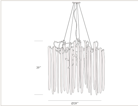
WATERFALL TORUS MEDIUM CHANDELIER CT3297-10 · Dia. 39" × 39" H
