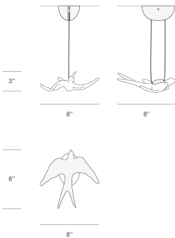
VOA GUTTURALIS MEDIUM PENDANT CT3415-1 · 8" W x 11" D x 3" H
