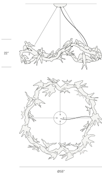
VOA HOOP LARGE CHANDELIER CT3424-23 · Dia. 55" × 22" H
