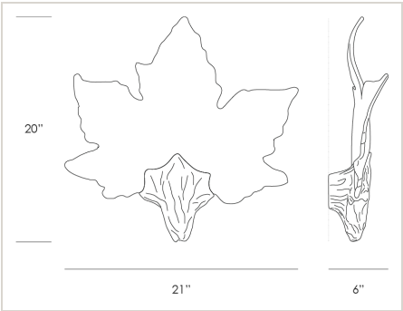
FOLIO PALM LARGE SCONCE AP1521-4 · 21" W × 6" D × 20" H
