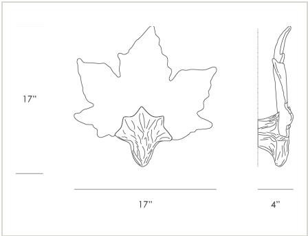
FOLIO PALM MEDIUM SCONCE AP1521-3 · 17" W × 4" D × 17" H
