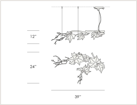
FOLIO BRANCH MEDIUM CHANDELIER CT3396-6 · 39" W x 24" D x 12" H
