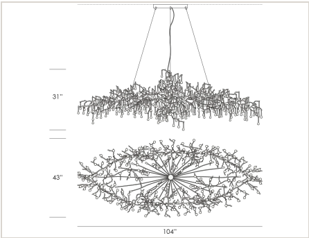
BIJOUT OVAL X-LARGE CHANDELIER CT3263-26 · 104" W x 43" D x 31" H
